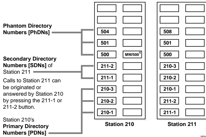
Figure 4 Multiple DNs
