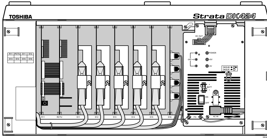
Figure 10 Base Cabinet Interior
