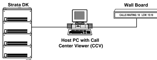
Figure 34 Direct Connection to DK424
