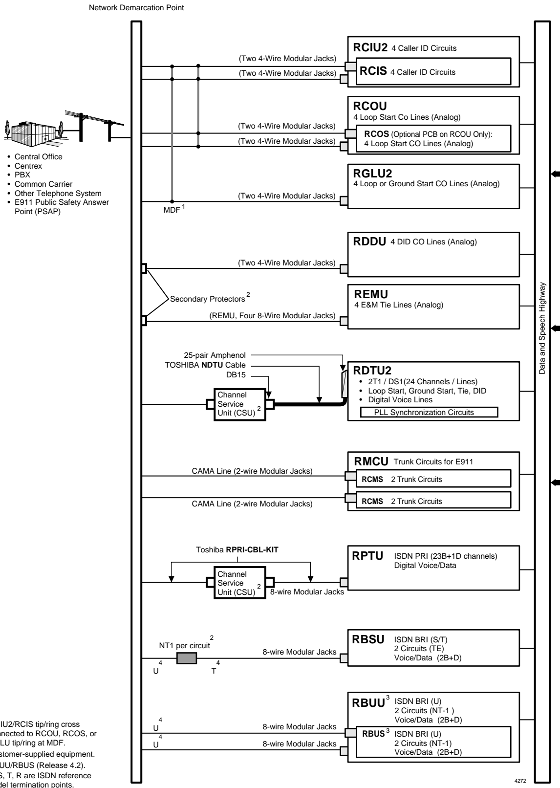
Figure 13 CO Line Side Functional Block Diagram
